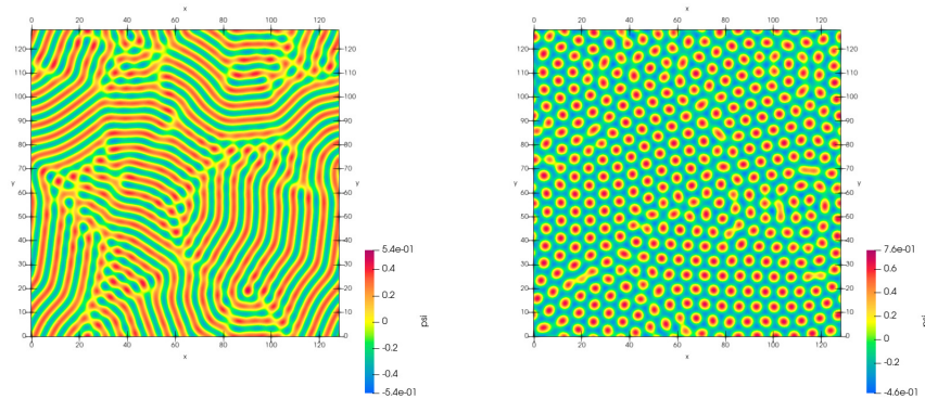
Figure 8.1: Solutions of the Swift-Hohenberg equation. Left: Roles ( \varepsilon = 0.1, A = 0.0 ); Right: Hexagons: ( \varepsilon = 0.1, A = 0.5 ). Array size is 256 \times 256 , with \Delta x = 0.5 length units (so, total area is 128 \times 128 unit length squared); critical wavelength is 2\pi per unit length (i.e. k_{\text{cr}} = 1 ; so around 20 roles or hexagons per 128 unit length should appear).
