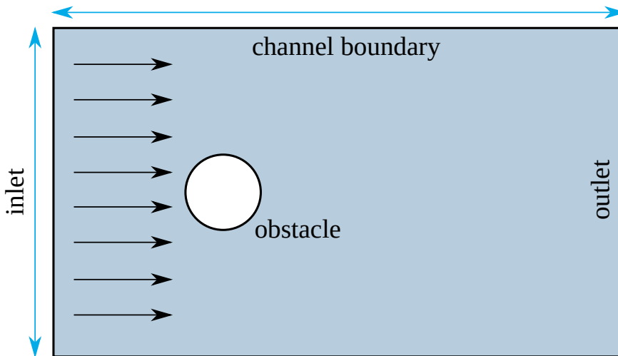
Figure 7.1: The Kármán case geometry with boundary labels.
