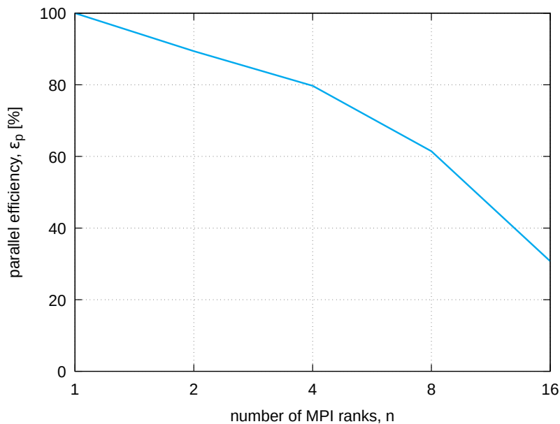
Figure 9.1: Kármán vortex sheet scaling plot – parallel efficiency as function of the number of MPI ranks used.
